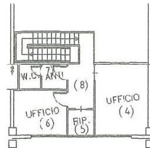
PIANO SOPPALCO
