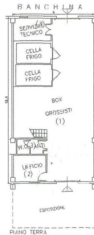
PIANO TERRA
